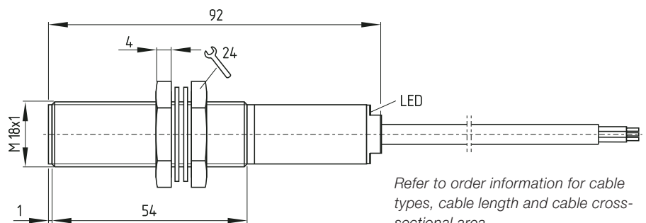
Dimensions of the CSS 180 Safety Sensor.
