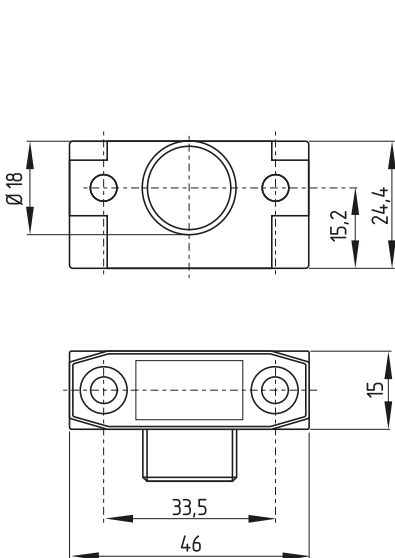
Dimensions of the CST Actuator.
