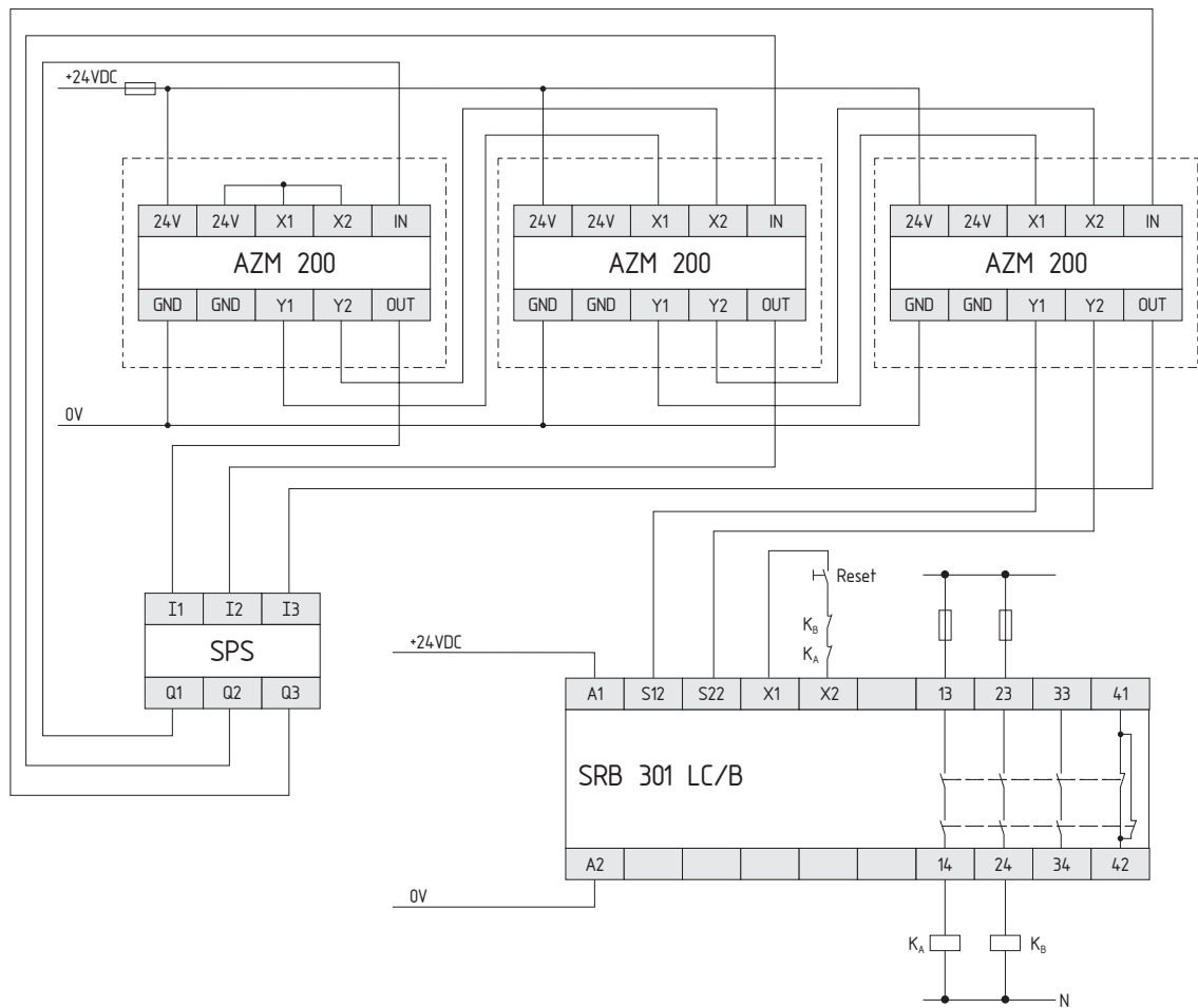
Wiring example: Series wiring of 3 AZM 200
