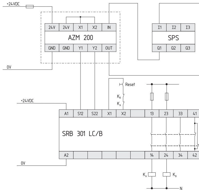
Wiring example: Single device wiring
